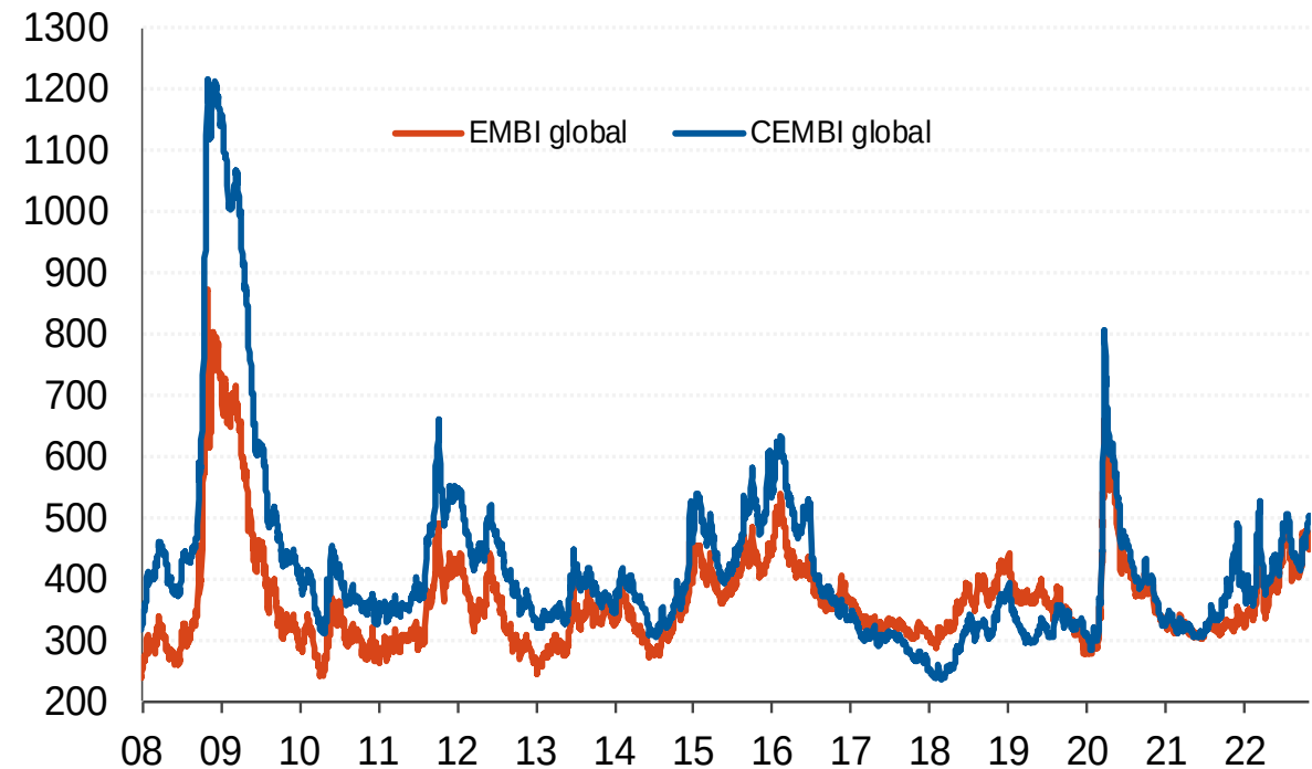
EMBI/CEMBI
